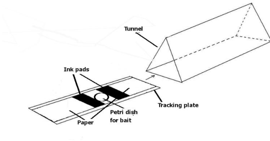
Figure 2. Schematic diagram of the footprint-tunnels to be used in this study.
